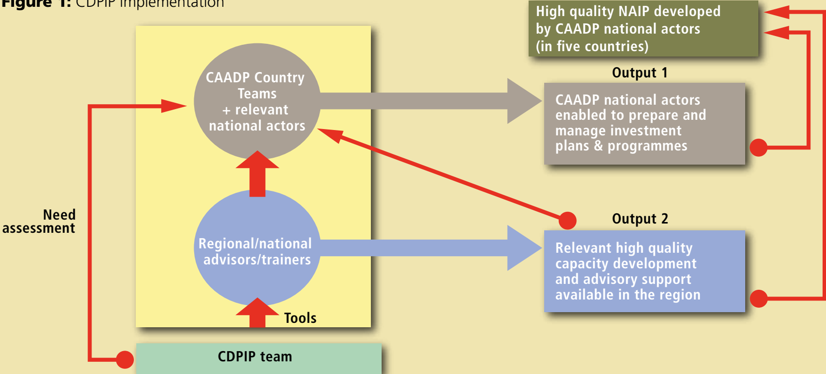
Figure 1: CDPIP implementation
