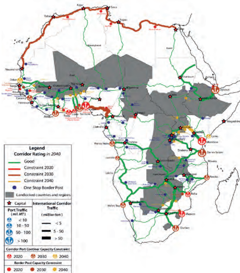
Figure 3.3 Forecast capacity gaps in ARTIN corridors
