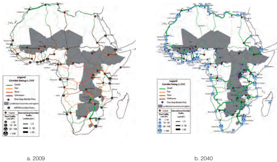
Figure 3.1 The ARTIN Corridors in 2009 and 2040
