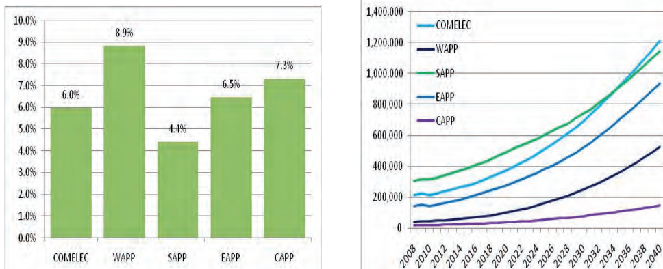
Figure 3.5 Annual growth rate (%) and increase in demand (in GWh) by power pool, 2011–40
